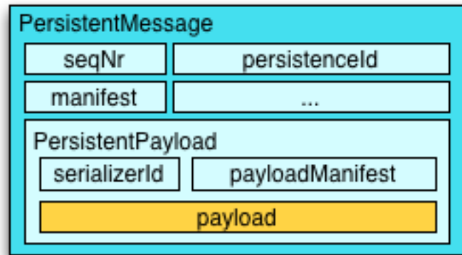
Figure 4.1: Akka Persistence provided serializers wrap the user payload in an envelope containing all persistence-relevant information. If the Journal uses provided Protobuf serializers for the wrapper types (e.g. PersistentRepr ), then the payload will be serialized using the user configured serializer, and if none is provided explicitly, Java serialization will be used for it.
