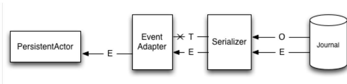
Figure 4.3: The serializer is aware of the old event types that need to be skipped (O), and can skip deserializing them all-together by simply returning a “tombstone” (T), which the EventAdapter converts into an empty EventSeq . Other events (E) can simply be passed through.
